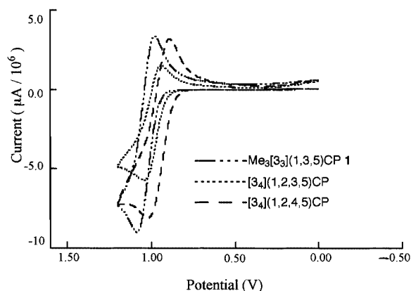
Figure 1. Cyclic voltammograms of [3 n ]cyclophanes in Cl 2 CHCHCl 2 (scan rate 20 mV/s)
