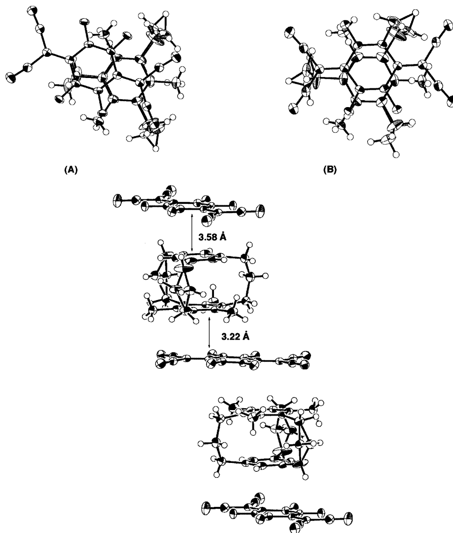
Figure 6. The crystal structure of the trimethyl[33](1,3,5)cyclophane (1)-TCNQ-F 4 (1:1) complex at -170\text{ }^{\circ}\text{C} : side views (A and B) and top view (C)
