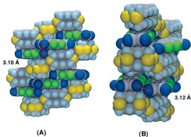
Figure 9. ORTEP drawings (CPK model) of the crystal packing diagram of trithia[3 3 ](1,3,5)cyclophane 4-TCNQ-F 4 (1:1) complex at -170 °C
