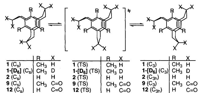
Scheme 2. Conformational isomerism of [3 3 ](1,3,5)cyclophanes by a bridge flipping process
