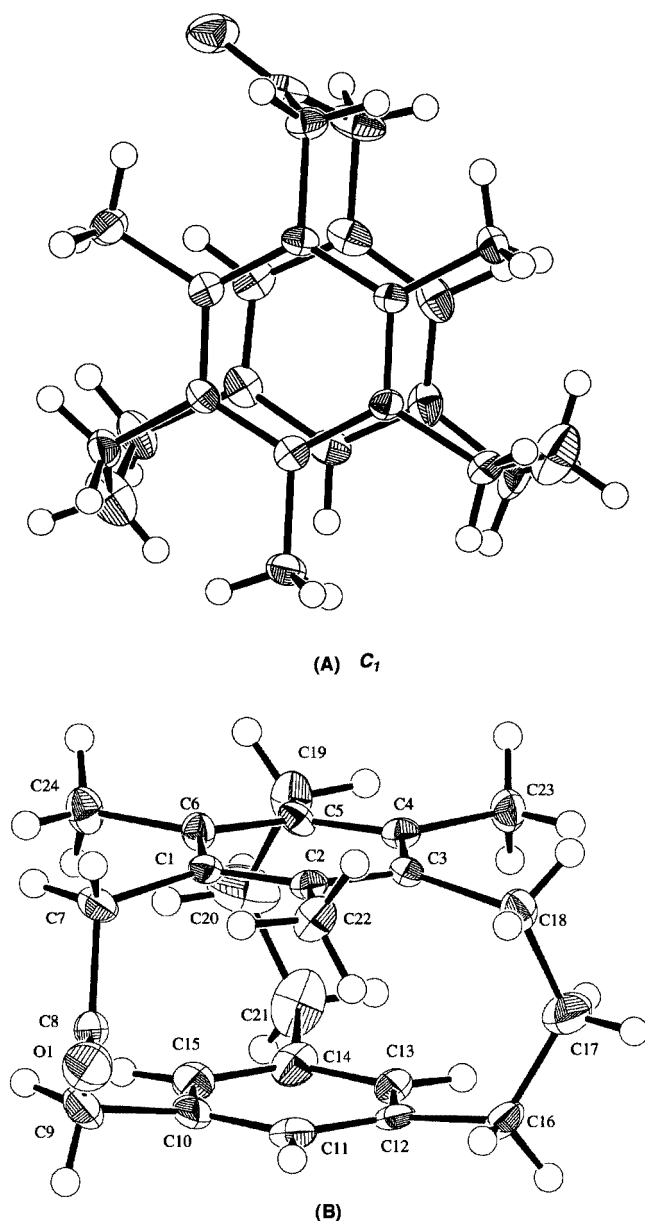
Figure 5. ORTEP drawings (A, top view; B, side view) of trimethyl-[3 3 ](1,3,5)cyclophane-2-one ( 10 ) at -170\text{ }^{\circ}\text{C} ; selected transannular distances [A]: C(1)–C(10) 3.099(8), C(2)–C(11) 3.154(8), C(3)–C(12) 3.084(8), C(4)–C(13) 3.170(8), C(5)–C(14) 3.093(7), C(6)–C(15) 3.170(8)
