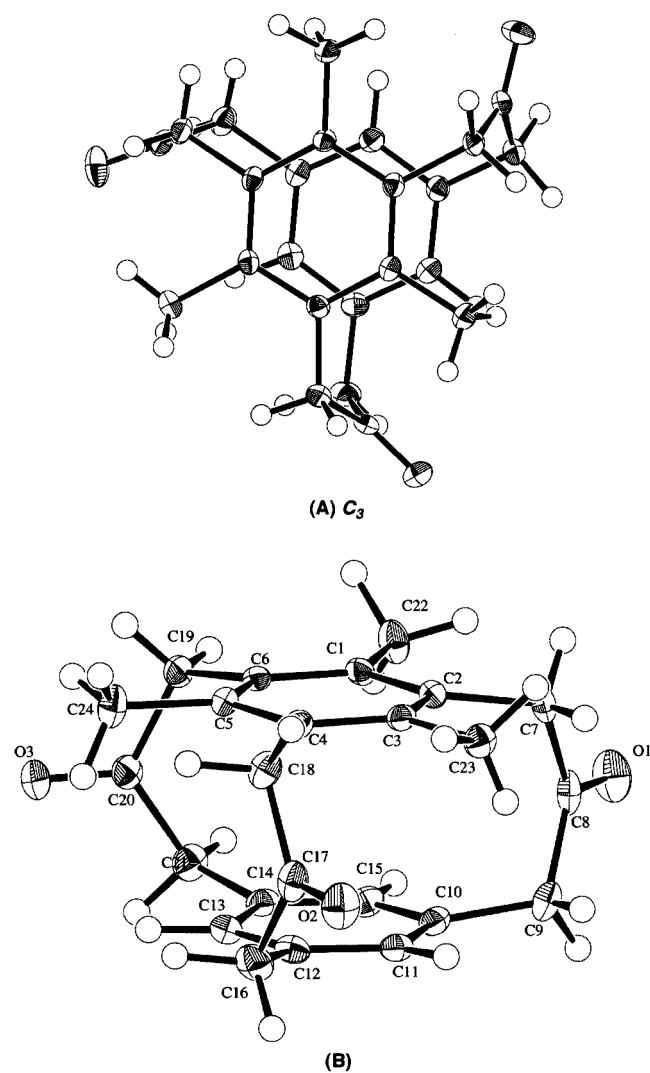
Figure 2. ORTEP drawings (A, top view; B, side view) of trimethyl- [3_3](1,3,5)\text{cyclophane-trione} ( 9 ) at -170^\circ\text{C} ; selected transannular distances [A]: C(1)–C(15) 3.140(2), C(2)–C(10) 3.079(2), C(3)–C(11) 3.137(2), C(4)–C(12) 3.079(2), C(5)–C(13) 3.142(2), C(6)–C(14) 3.083(2)
