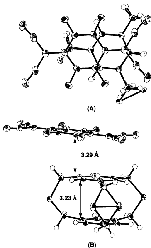
Figure 8. The crystal structure of the trithia[3 3 ](1,3,5)cyclophane 4-TCNQ-F 4 (1:1) complex at -170 °C (A, top view; B, side view)
