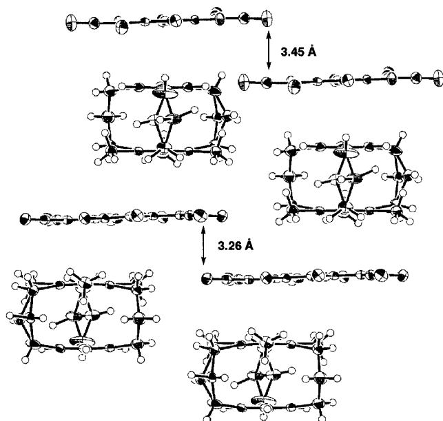
Figure 7. The crystal packing diagram of the trimethyl[3 3 ](1,3,5)-cyclophane (1)-TCNQ-F 4 (1:1) complex at -170 °C
