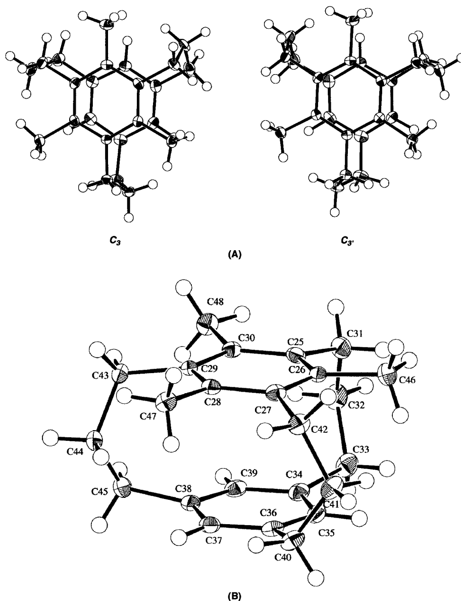
Figure 4. ORTEP drawings (A, top view; B, side view) of trimethyl[3 3 ](1,3,5)cyclophane ( 1 ) at -170\text{ }^{\circ}\text{C} ; selected transannular distances [A]: C(1)–C(10) 3.072(3), C(2)–C(11) 3.137(4), C(3)–C(12) 3.087(4), C(4)–C(13) 3.173(4), C(5)–C(14) 3.097(4), C(6)–C(15) 3.160(4), C(25)–C(34) 3.090(3), C(26)–C(35) 3.145(3), C(27)–C(36) 3.081(3), C(28)–C(37) 3.158(3), C(29)–C(38) 3.096(3), C(30)–C(39) 3.157(3)
